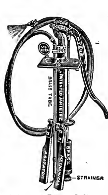
Myers' Barrel Spray Outfit No. 318B
