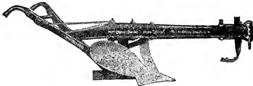
Oliver No. 1 Road and Grading Plow
