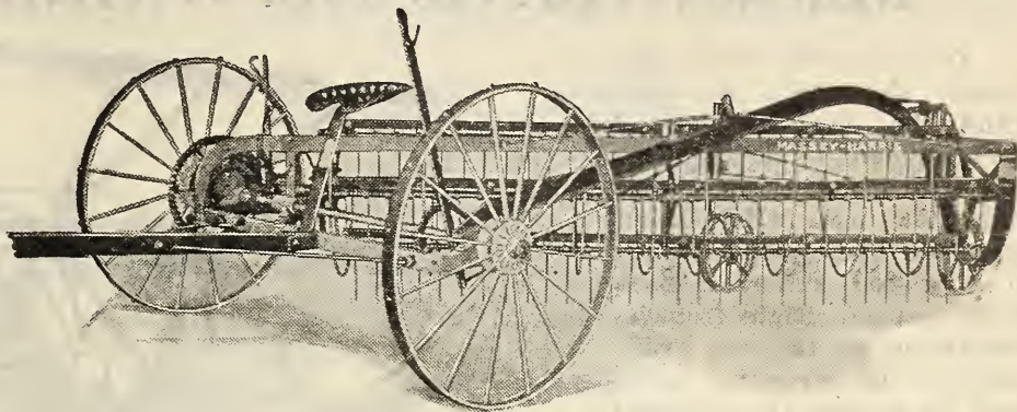
9 1-2 Foot Cylinder for Hay.
