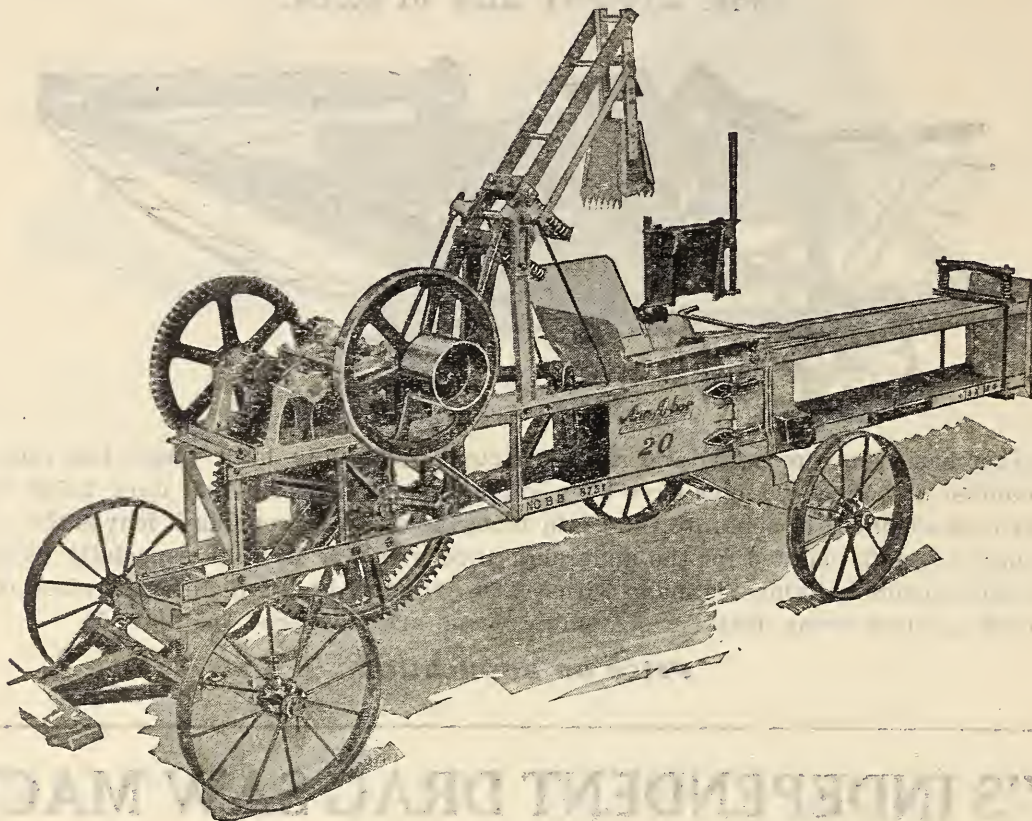
THE ANN ARBOR "20."
