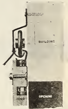
Sectional View, No. 2 "GLIDE" HANGER AND TRACK.
