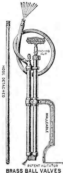
BRASS BALL VALVES
