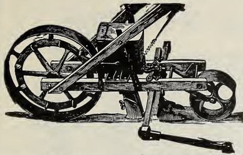
New Model Seed Drill. Will sow anything from every Seed to Peas and Beans perfectly.
