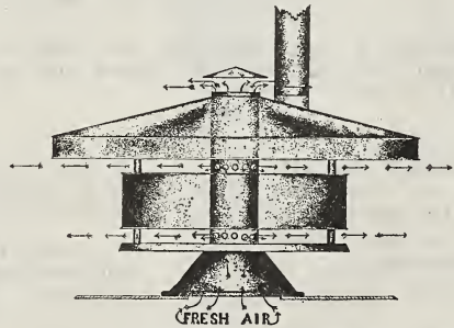
Skeleton of No. 2-B and No. 4-B Types Showing Fresh Air Intake and Heat Distribution
