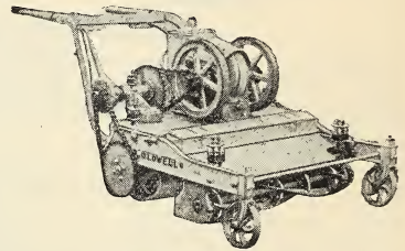
Coldwell Lawn Mower
