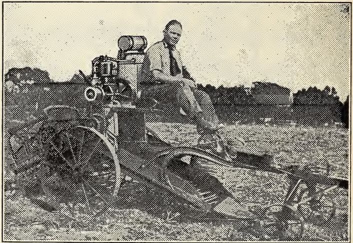
Four-Horsepower Cushman Engine on a Hoover Digger
