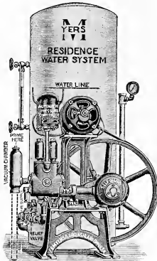
Myers Electric House Pump
