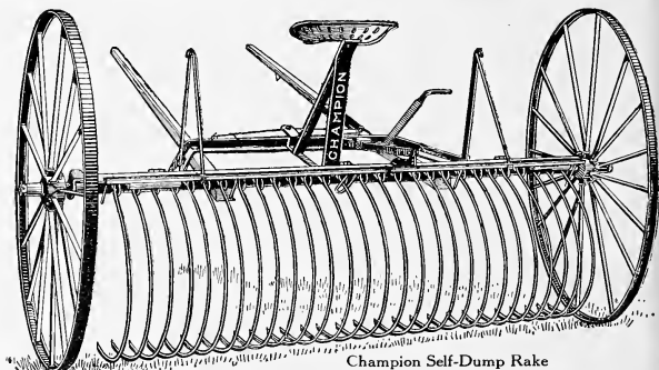
Champion Self-Dump Rake
