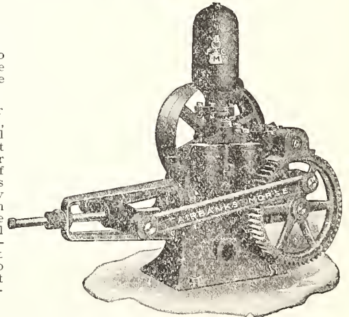
Sizes and Capacities of Typhoon Double-Acting Power Pumps--Belt Driven
