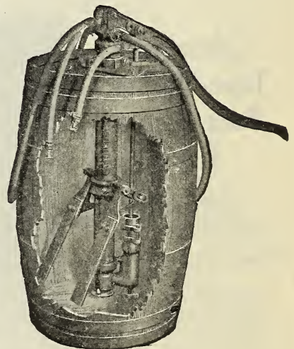
Pomona Spray Pump
