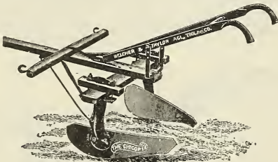
THE SHOVEL POTATO HOE
