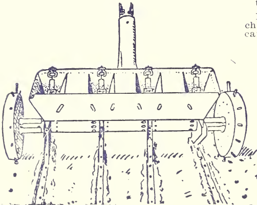
No. 1A. Extra Arbor for very small and very large seeds. Price, $0.40.
