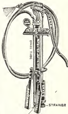
BAT JET AGITATOR
