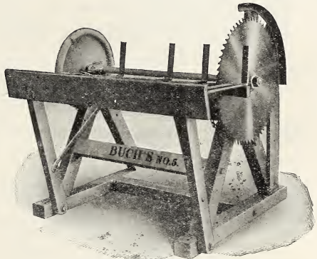
Saw Frames, $17.50 to $27.50 Circular Saws, from $4.50 to $8.50 according to size
