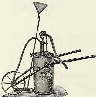
12 Gallons on Wheels, $22.50
