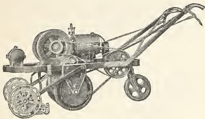
Ideal 30-inch Power Mower
