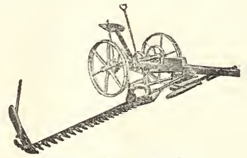
Avery 5 ft. Champion Mower.
