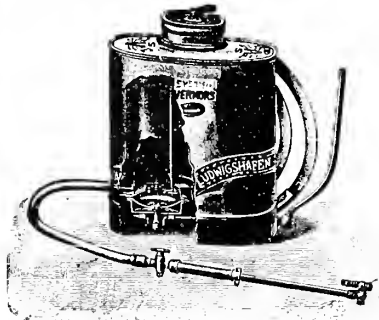
Vermor Knapsack Sprayer
