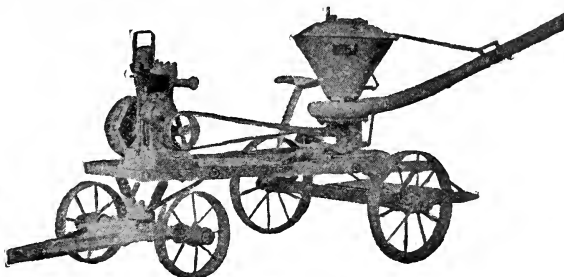
Bean's Power Duster
