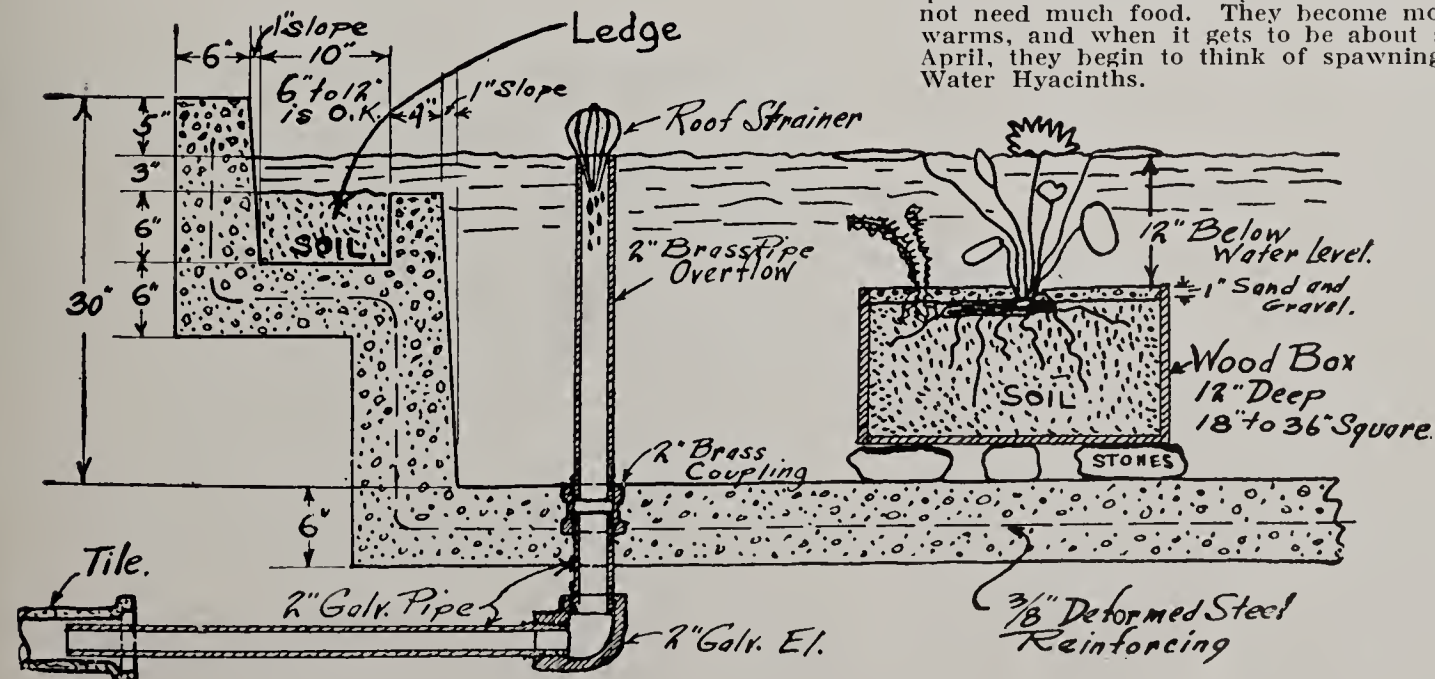
This sectional drawing shows the construction of a well-reinforced concrete pool for lilies and Goldfish. The Ledge can be constructed on one or more sides of the pool, depending on effect desired. It is built to accommodate the floating plants (Water Hyacinths, etc.) and the shallow water plants (Cattail, Pickerel Rush, Water Canna, etc.). Where no ledge is provided, soil boxes, buckets, etc., properly arranged, will give a good effect.
