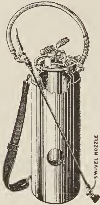
BROWN'S OPEN-HED Four Gallon Tank—Compressed Air 5 in. Opening Galvanized Steel, $5.50—Brass, $9.00 Complete as Shown Above
