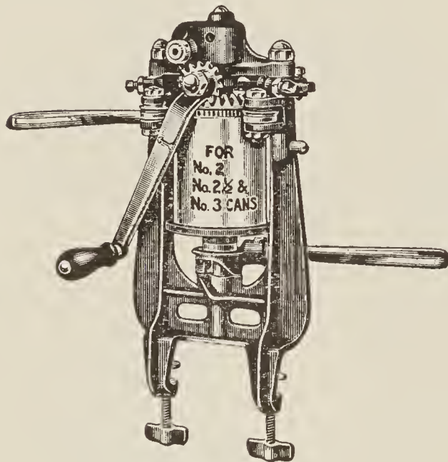
NATIONAL SEAL-O-MATIC Handles No. 2—2½—3 Seals, cuts and re-conditions. $11.50 delivered
