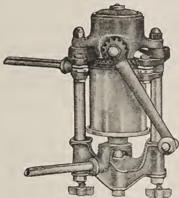
THE NATIONAL SEAL-O-MATIC High Speed Handles No. 2, 2½ and 3 $12.50, Delivered Seals, cuts and re-conditions
