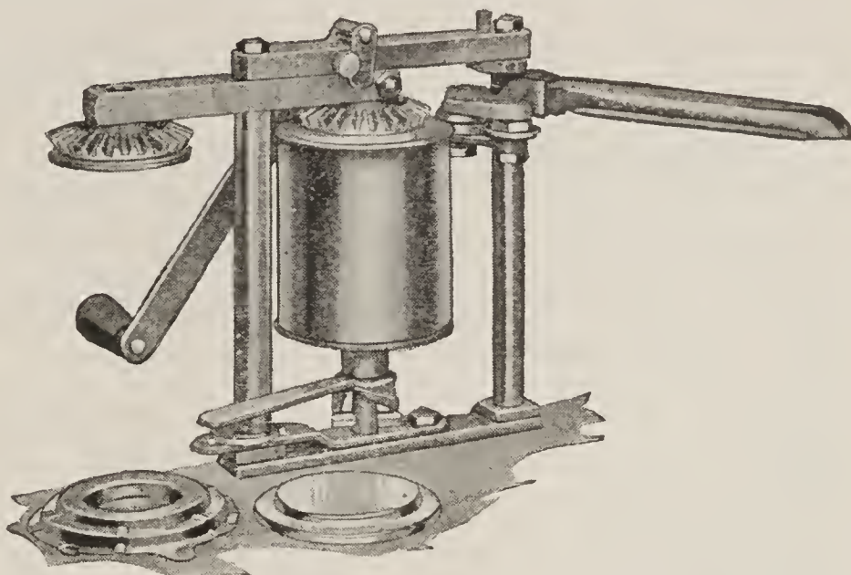
QUICK CHANGE BURPEE Handles No. 2 and No. 3 $12.00, Delivered Seals, cuts and re-conditions
