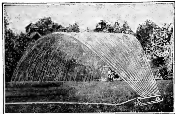
The Waterfan Sprinkler in operation
