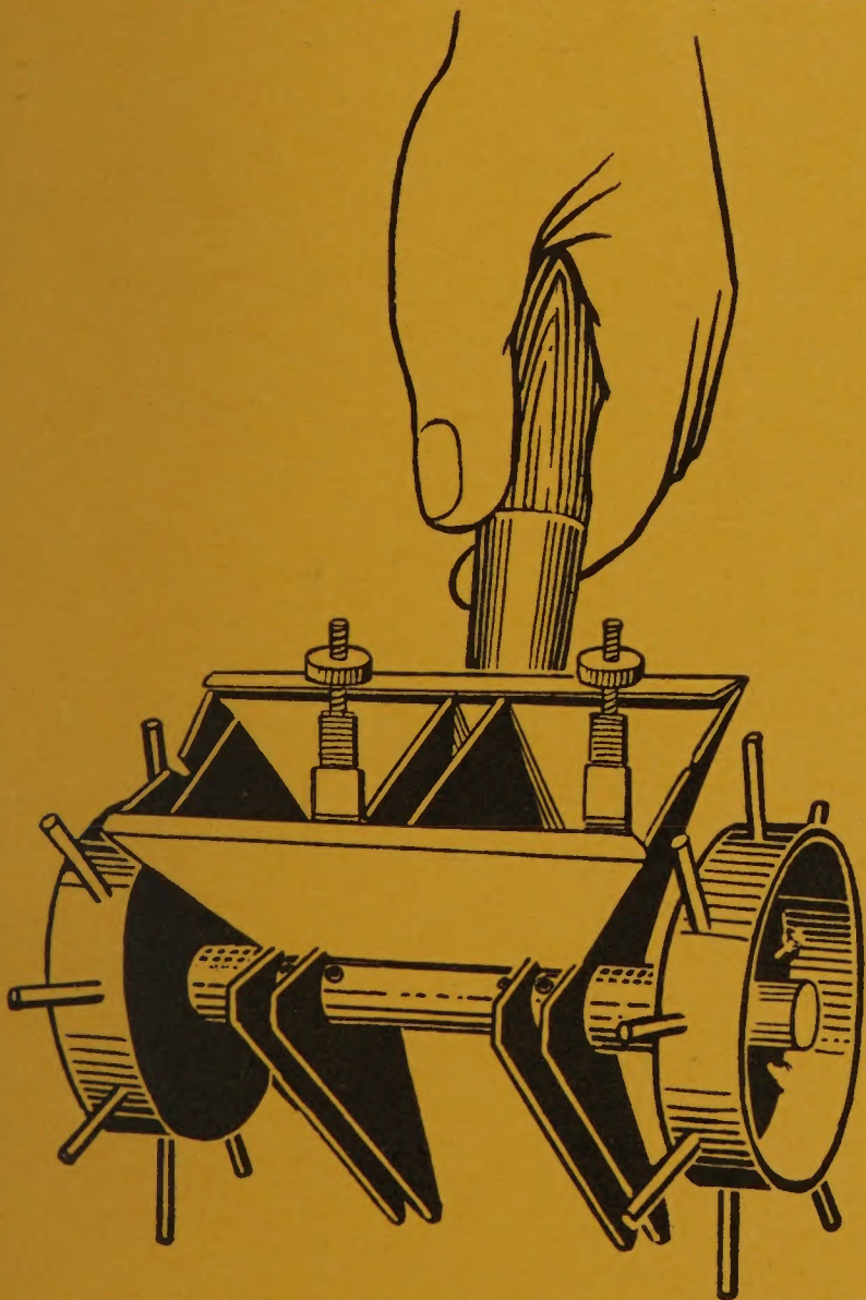
2-Row Seeder is about 6 inches long and seeds 2 rows 2¼ inches apart. Price.....$4.50
