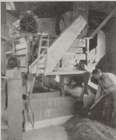
2. Suspended sieve trays separate the coarse material from the seed and fine chaff allowing the seed to fall on clean canvas.
