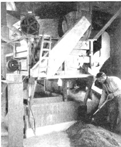
2. Suspended sieve trays separate the coarse material from the seed and fine chaff allowing the seed to fall on clean canvases.
