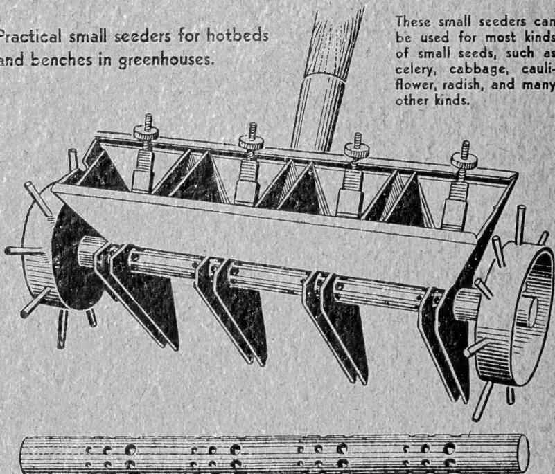
4-Row Seeder. This machine is about 10 \frac{1}{2} inches long and seeds 4 rows 2 \frac{1}{4} inches apart. Price.....$6.50
