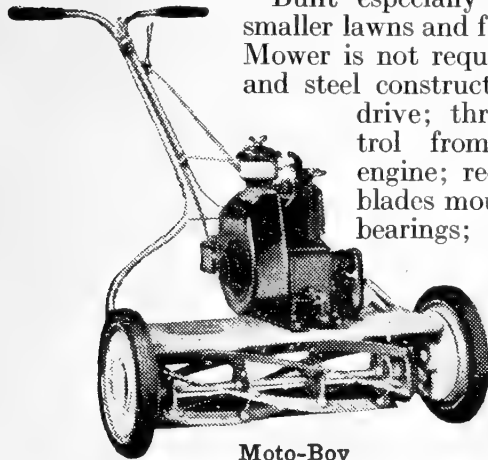
Moto-Boy Model Moto-Mower
