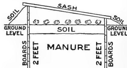
Showing the construction of a small hot-bed.
