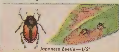
Japanese Beetle—1/2"
