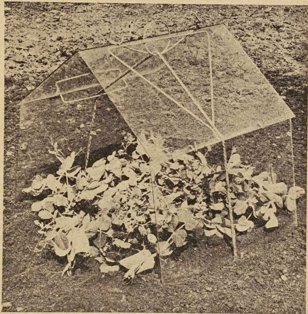
The Chase P.M.G. is 18 inches long, 20 inches wide and 16 inches high to the ridge.
