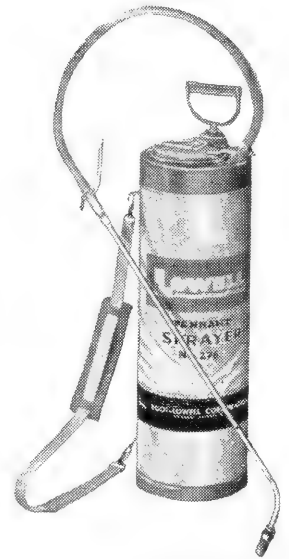
No. 276 Pennant Root-Loell Sprayer. 4 gal. capacity galv. tank, 7½x22 in. New "seal-tight" finger tip locking cover. New "Any-Spray" nozzle. A sprayer that is completely safe and fool proof. Can be used for any spraying job.
