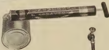
No. G-10 Bug-O-Gun Tank capacity about 1¾ gals. Constructed of heavy galvanized steel. Has attached funnel. Pump 6 inches seamless brass tubing, 12-inch brass extension rod. Nozzle can be detached. 20-inch durable spray hose. Web carrying strap. Heavy forged brass, leak-proof release valve. Weight about 7 lbs. Price, $7.50 each.
