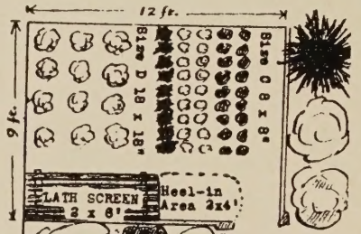
LAYOUT PLAN MINIMUM-SIZE HOME NURSERY
