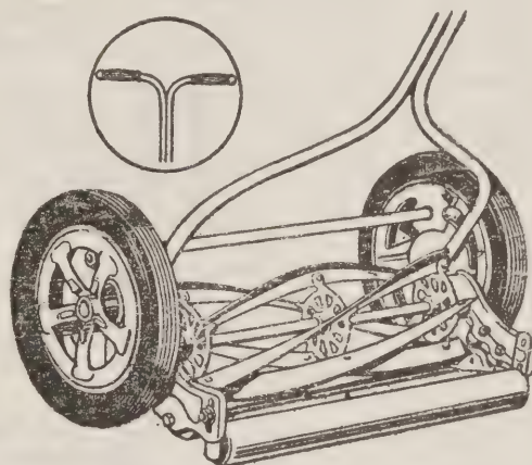
Schell's Special Hand Mower
