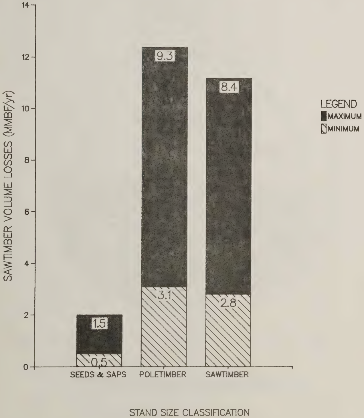
FIGURE 4. Distribution of projected annual volume losses by size class for the Tonto National Forest
