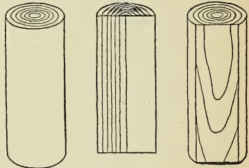
FIG. 11.—Annual rings.
