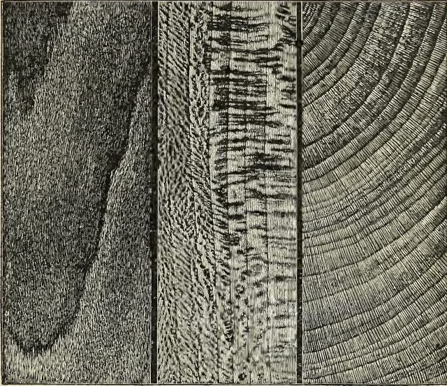
FIG. 10.—Wood of Western Hemlock.
