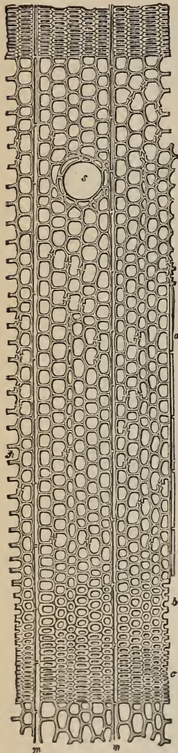
FIG. 9.—Wood of a spruce, greatly magnified.
