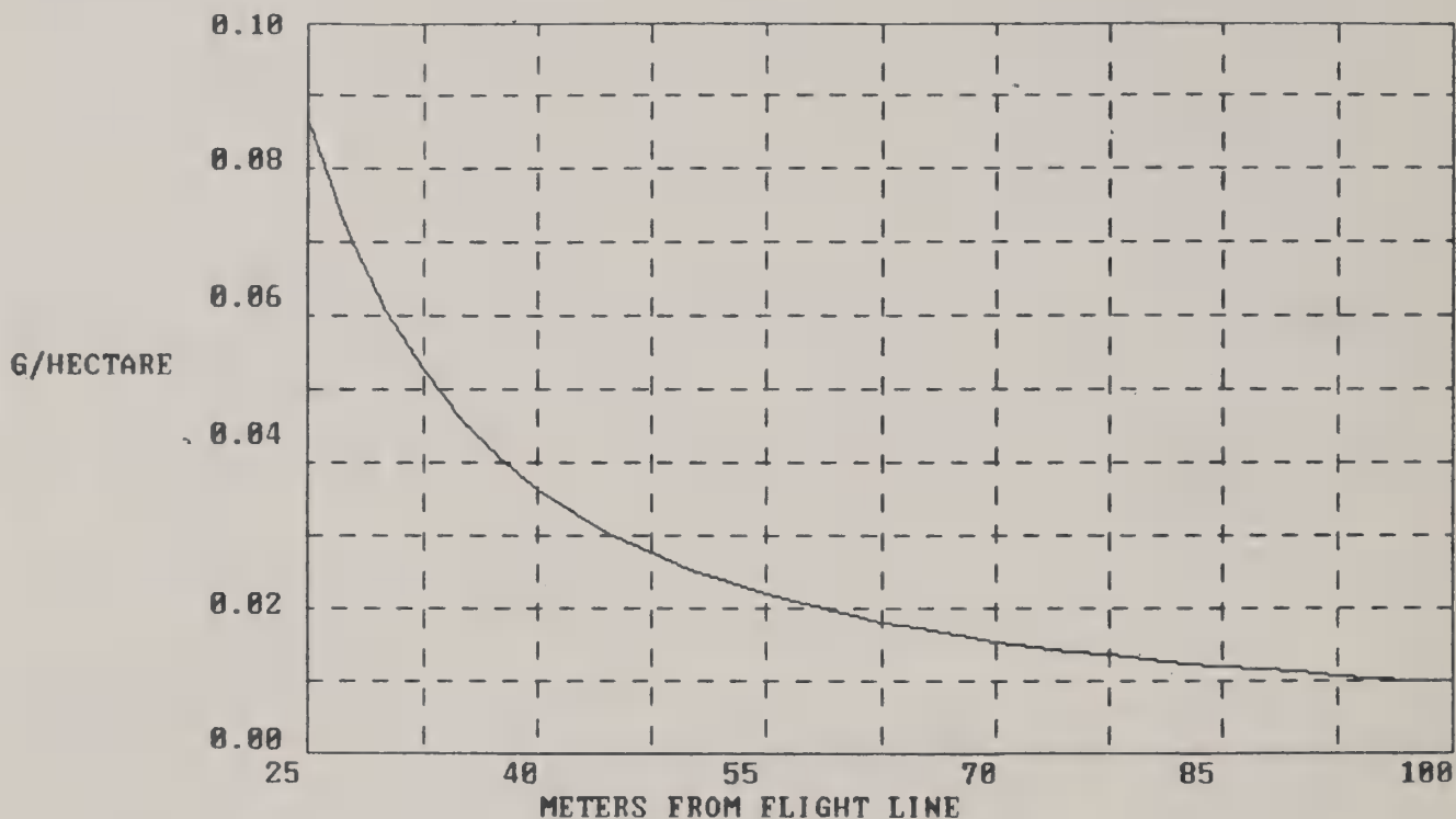
Figure 4-3--Spray deposition downwind of a right-of-way--aerial application at 1.12 kg/ha with a microfoil boom
