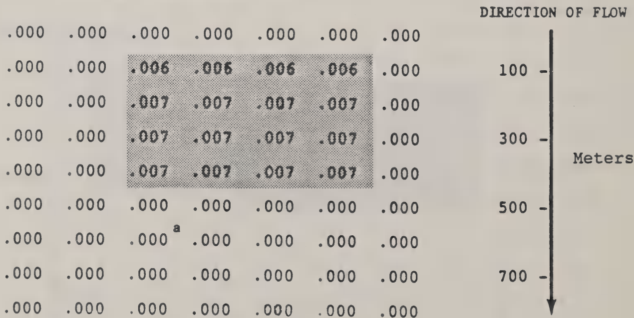
Figure 4-21--Two-dimensional ground water model predictions for picloram at 0.2 years in Florida near-surface aquifer, steady flow. Initial concentration (ave.) under treated area is less than 0.001 ppm.
