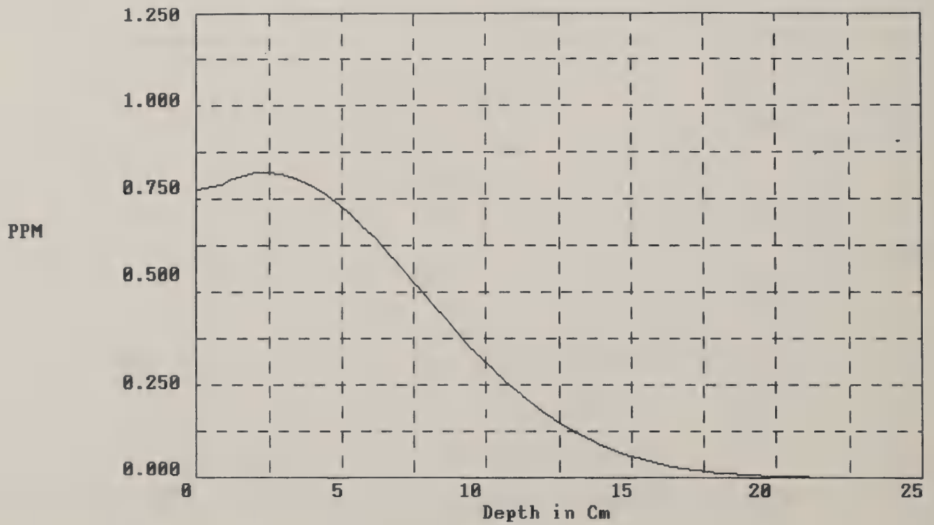
Figure 4-13--Leaching profiles of picloram in sandy loam soil after 6 cm of percolated water
