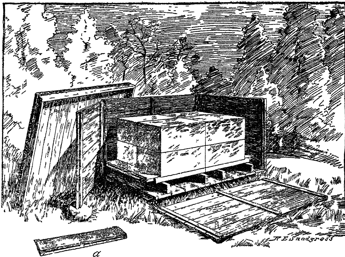
FIG 2—The winter packing cases used in the Bureau of Entomology apiary. a , Detail of tunnel to hives. In the specifications given in this bulletin (p 9) provision is made for room for a third hive body to be added in the spring.
