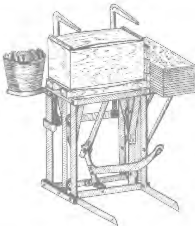
Fig. 24. Bar Nailing Press.
