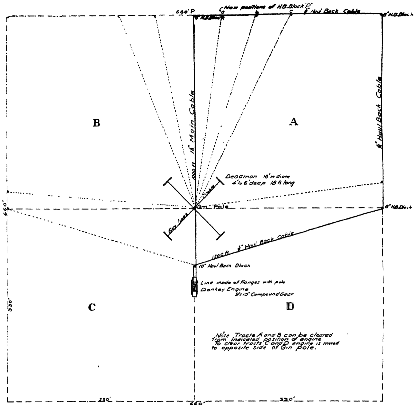
PLAN Showing Position of Donkey Engine and Rigging for Clearing a Ten Acre Tract scale 1"=50'
