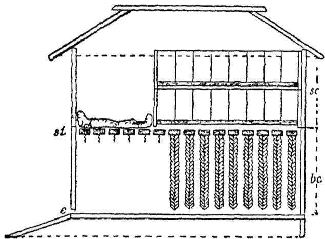
Fig. 5. The Simmins Nonswarming System—Single-story Hive with Supers bc, brood chamber; sc, supers; st, starters of foundation; e, entrance.
