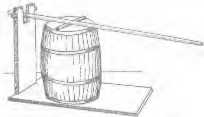
Fig. 5. A Good Home-made Lever Barrel Press.
