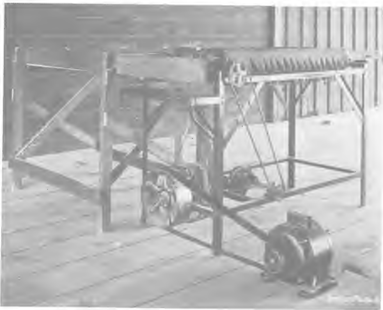
Fig. 12. Apple Wiping Machine. Courtesy Enterprise Fruit Machine Co., Zillah, Wash.
