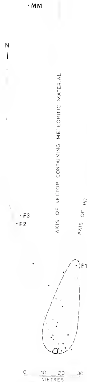
Figure 2.—Field distribution of the main mass (MM), major fragments (F1-F3), and minor fragments (indicated by dots) of the Haig meteorite relative to its impact pit. Limestone fragments ejected from the pit are enclosed within the broken line.
