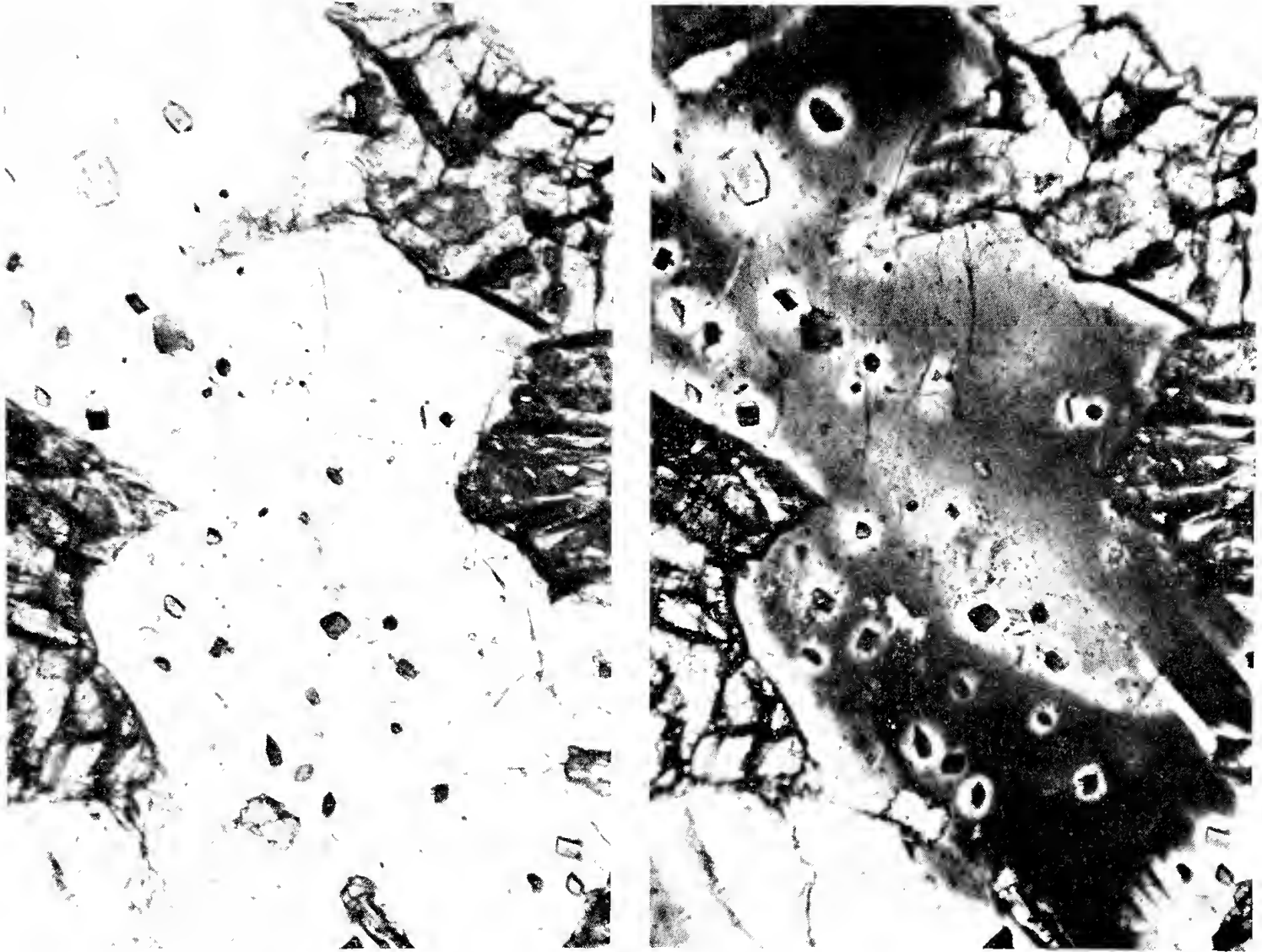
Figure 2.—A (left) Photomicrograph of a plagioclase grain (white) in Spec. 16311 showing euhedral spinel inclusions (shades of dark grey). The other dark mineral is clinopyroxene which contains some vermiform spinel inclusions. Plain light, X80. B (right)—Same field of view as Figure 2A with nicols crossed. Note the andesine haloes around spinel inclusions in the labradorite host.
