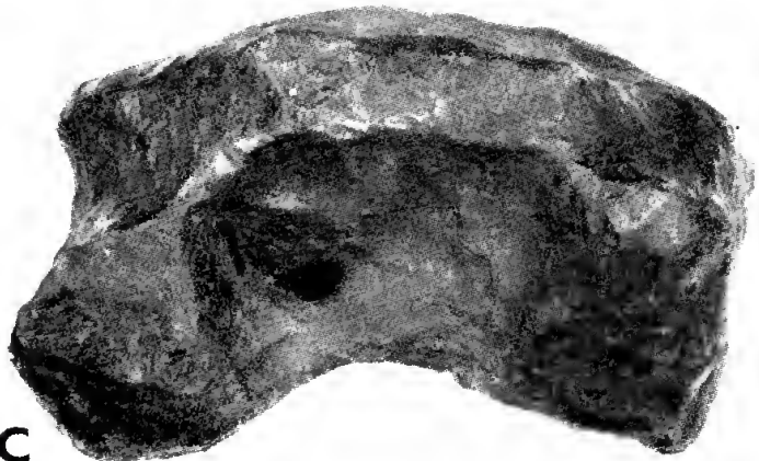
Figure 2.—Yarri meteorite. Scale bar in centimetres. A.—Convex face. Hammer dents, artificial damage and cut at lower end. B.—Side elevation (left side of A). C.—End elevation (upper end of A).
