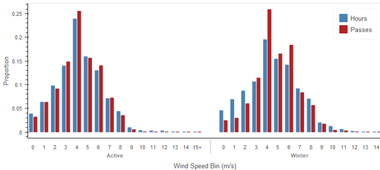
Figure 8. A comparison of background windspeeds recorded at the BAFM8 station (blue) and those recorded during bat passes (red). Where the bars showing passes exceed hours, bat activity is higher than expected for this wind speed bin.
