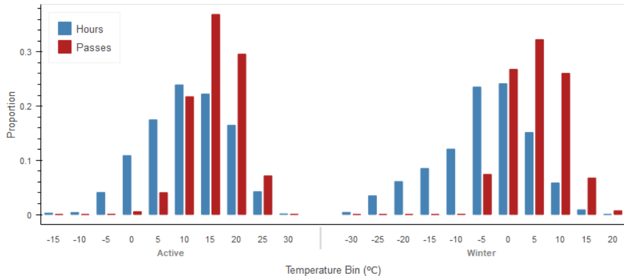
Figure 6. A comparison of average temperatures during bat passes (red) and average hourly background temperatures (blue) recorded at the BAFM8 station, located 22.4 km to the southeast of the detector. Where the bars showing passes exceed hours, bat activity is higher than expected for this temperature bin.
