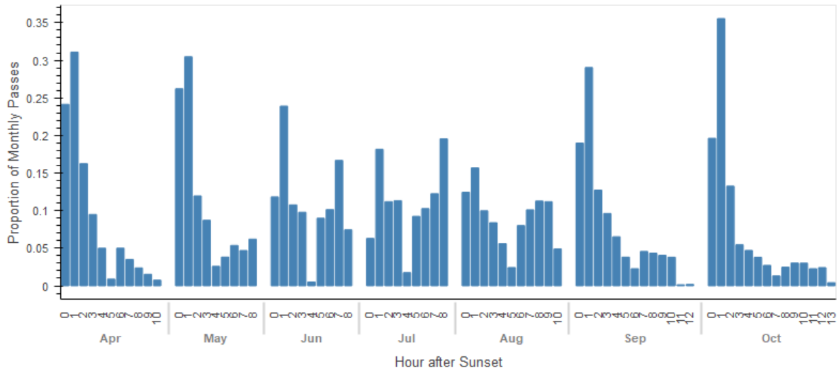
Figure 4. Average nightly activity of bats recorded at the Big Sky Mine Pond B-9 acoustic monitoring station across the active season.
