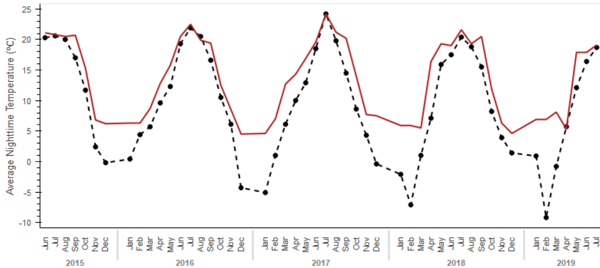
Figure 5. Average bat pass temperatures (red line) and average background temperatures (black line) across the year at the Big Sky Mine Pond B-9 detector.
