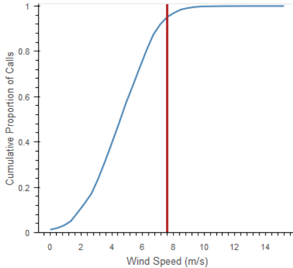
Figure 7. The cumulative sum of wind speeds recorded at the BAFM8 station during bat passes. The speed at which 95% of all activity occurs at or below is highlighted in red.
