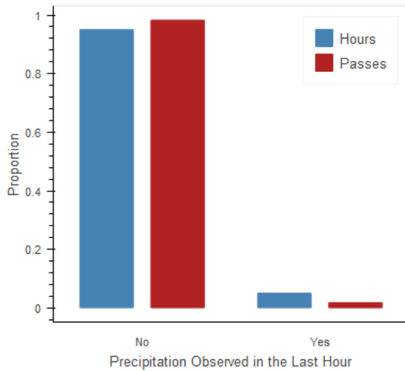
Figure 10. A comparison of hours with and without precipitation for bat passes (red) and all nighttime hours (blue) during the active season as recorded at the BAFM8 station, located 22.4 km to the southeast of the detector. Where the bars showing passes exceed hours, bat activity is higher than expected for this precipitation bin.
