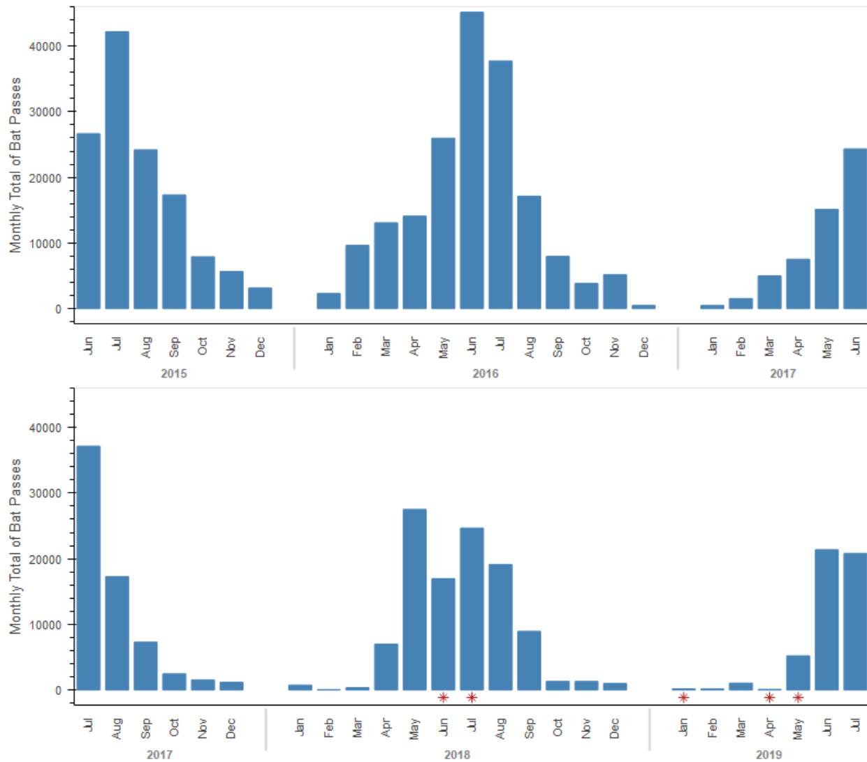
Figure 3. Total monthly bat passes recorded at the Big Sky Mine Pond B-9 acoustic monitoring station. Months marked with an asterisk should be interpreted with caution as those data may not represent valid trend due to data collection for only part of that month, equipment malfunction or other issues.
