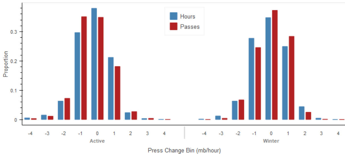
Figure 9. Hourly changes in background barometric pressure at the K1S3 station (blue) compared to changes in pressure when bat passes were recorded (red) at the Big Sky Mine Pond B-9 detector. Where the bars showing passes exceed hours, bat activity is higher than expected for this pressure change bin.
