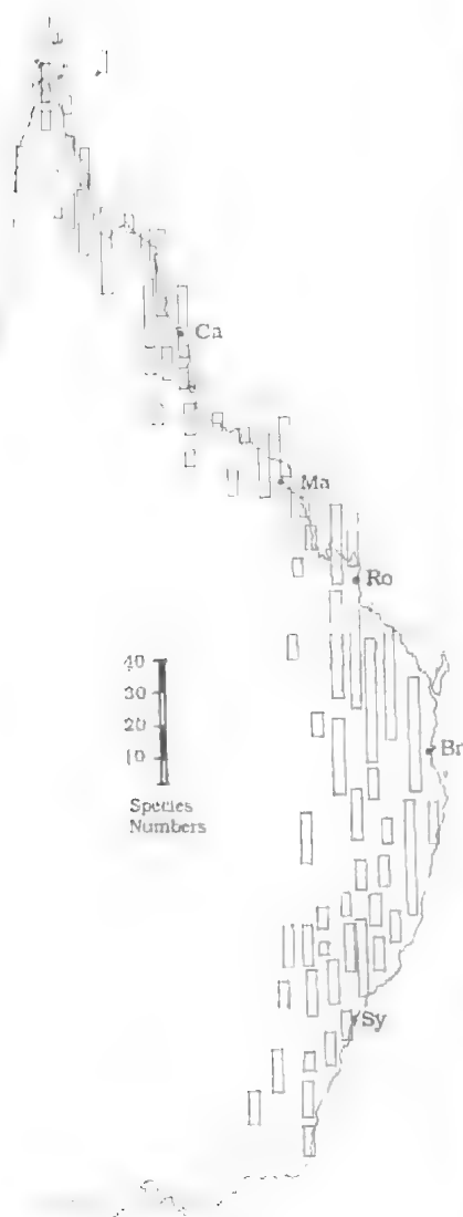
FIG. 3. Comparison of land snail diversity levels at selected sites in eastern Australia (Ca, Cairns; Ma, Mackay; Ro, Rockhampton; Br, Brisbane; Sy, Sydney).
