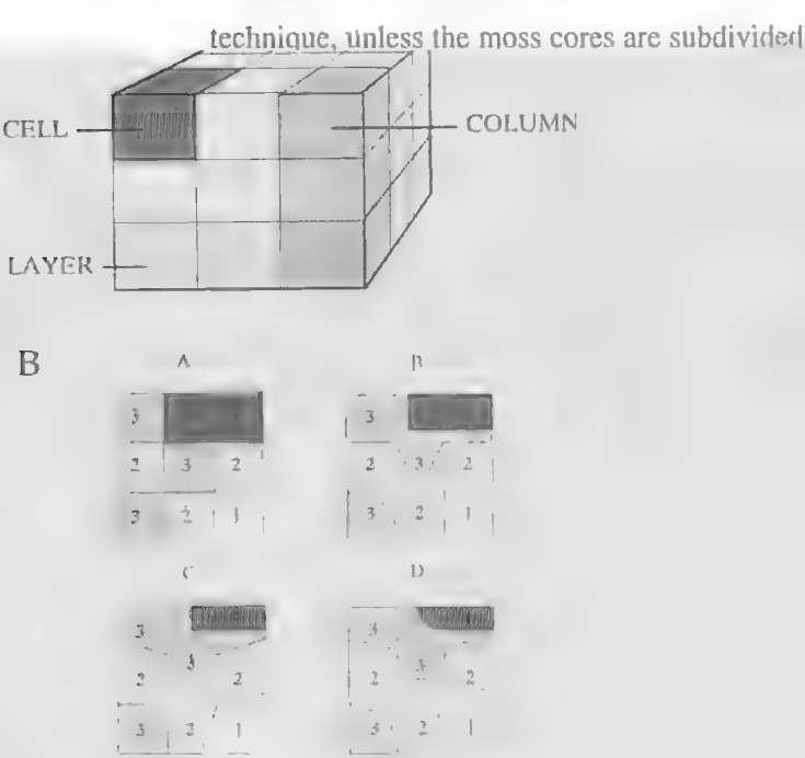
FIG. 2. A. Terminology used for describing parts of the 10×10×5cm sample of Antarctic moss. B. Illustration of the process of smoothing used in constructing the distributional patterns of four species of tardigrades inhabiting the volumetric sample of Antarctic moss. Top face of sample is illustrated; numbers indicate the number of species in each column (see text for details).
