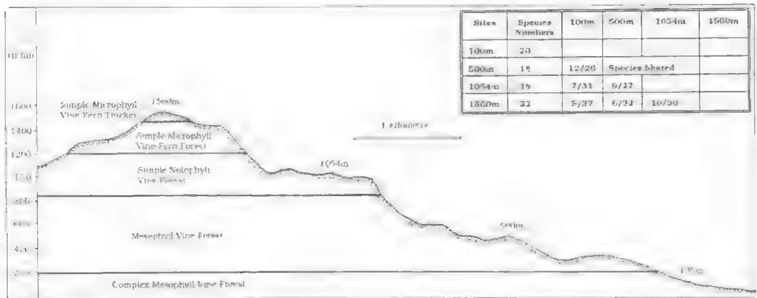
FIG. 4. Altitudinal stratification of land snail communities on Mt Bellenden Ker, NEQ (12/26 means that a total of 26 species were collected at 100m/500m sites and 12 were common to both).
