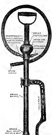
Spray and Whitewash Pump
