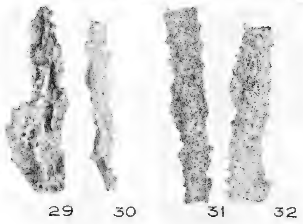
Sandruba Fulgurites, natural size
