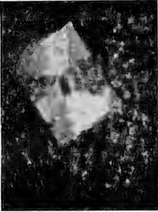
Fig. 2 Enlargement of cross section in top left-hand corner of above showing replacement of chialstolite by quartz and sericite. Crossed Nicols x 56.
