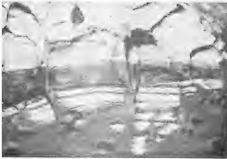
Fig. 1 Granite intruded along bedding of Willyama metasediments— Brewery Creek.
