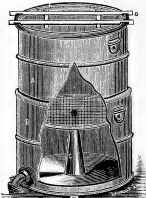
DADANT'S UNCAPPING-CAN.
