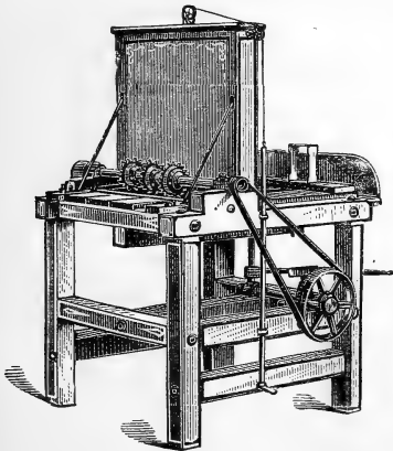
GRAY'S IMPROVED MACHINE FOR MAKING SECTIONS.
