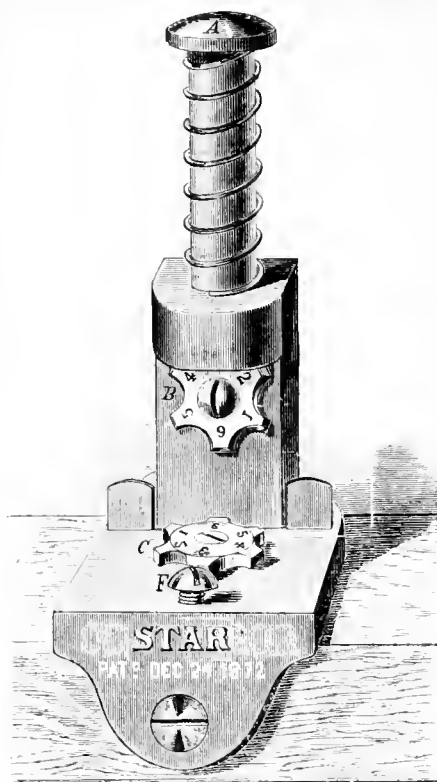
STAR SAW-SET FOR HAND, BACK, BAND, WEB, WOOD, AND SMALL CIRCULAR SAWS, NOT THICKER THAN IS GAUGE.
