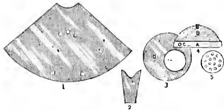
THE TINWORK USED FOR COLD-BLAST SMOKER.
