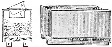
McINTYRE'S UNCAPPING-BOX.
