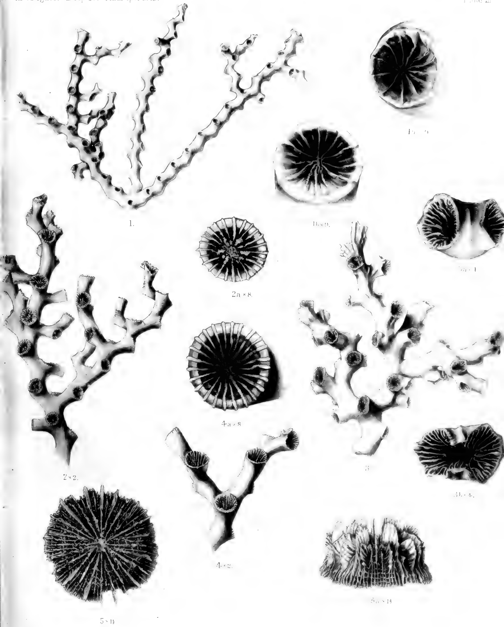
1. Lophohelia investigatoris .
