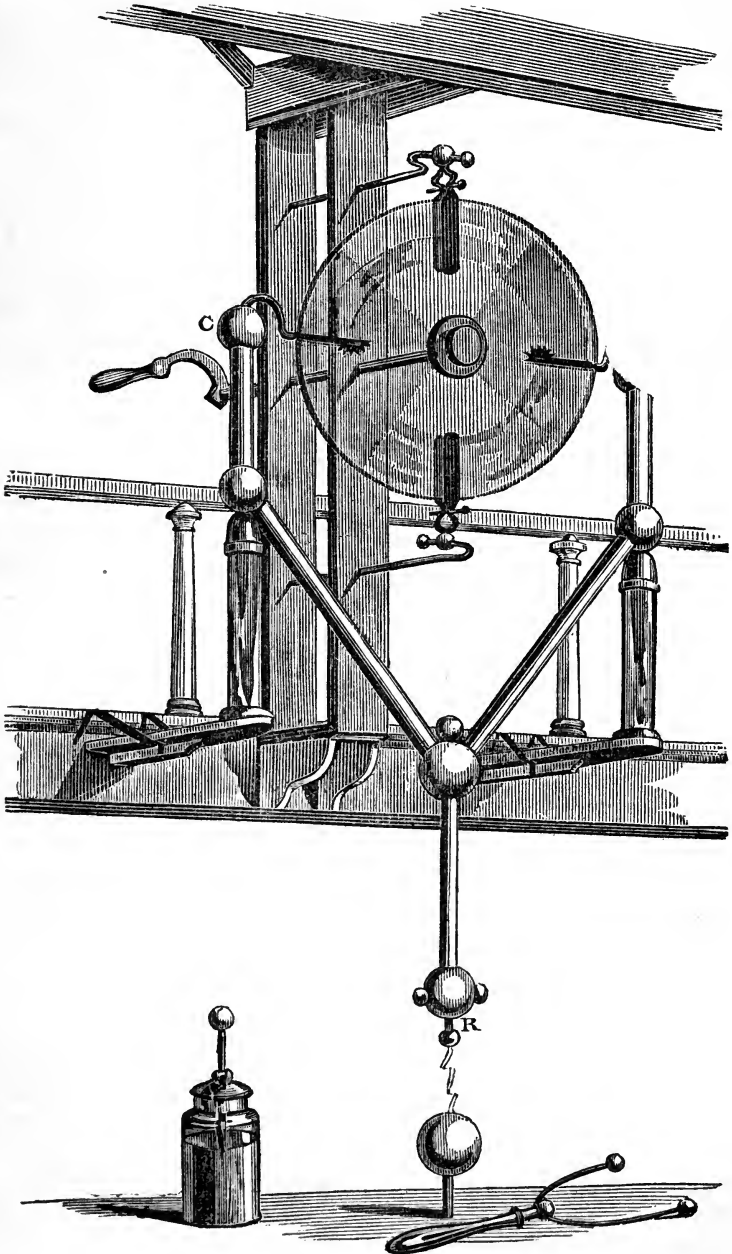
HARE'S ELECTRICAL MACHINE.
