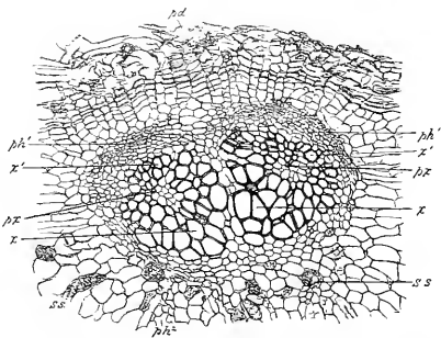
Fig. 7. Lyginodendron oldhamium . Double leaf-trace bundle and adjacent tissues in transverse section. x centripetal; x' centrifugal xylem; px protoxylem; ph phloem of bundles; ph' part of phloem of stele; ss secretory sacs; pd part of periderm. \times about 40. WILLIAMSON Coll n 1884.
