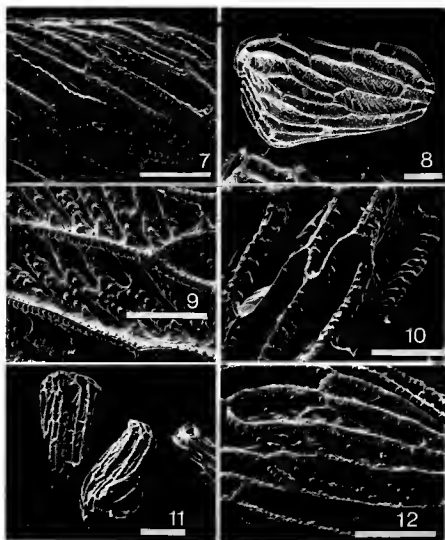
Pl. 2. — Striga densiflora (74-1): 7, detail of surface; in this species the regions between the ridges are only sparsely ornamented; scale = 50 \mu m. — Striga euphratoides (67-1): 8, this species has very distinct surface features, especially of the secondary ridges; scale = 100 \mu m; 9, detail of the secondary ridges showing the conspicuous protuberances; scale = 50 \mu m. — Striga forbesii (78-3): 10, the ornamentation of the primary ridges is obscure with short, blunt protuberances; scale = 50 \mu m. — Striga gesnerioides (79-1): 11, general view; scale = 100 \mu m; 12, note scattered protuberances on secondary ridges; scale = 50 \mu m.
