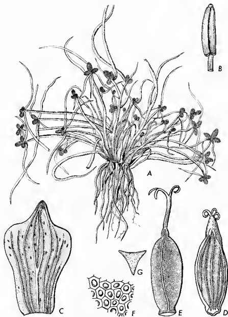
Pl. 1. — Lipocarpa raynleana Govindarajalu : A, habit \times \frac{1}{2} ; B, stamen \times 30 ; C, glume, dorsal view \times 10 ; D, squamella \times 13 ; E, nut \times 15 ; F, surface view of epicarpic cells (diagrammatic); G, transection of nut (diagrammatic). — Based on Govindarajalu 14948, type.
